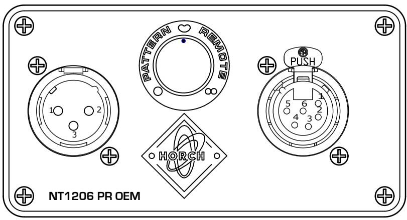
3 pol XLR CONNECTOR
